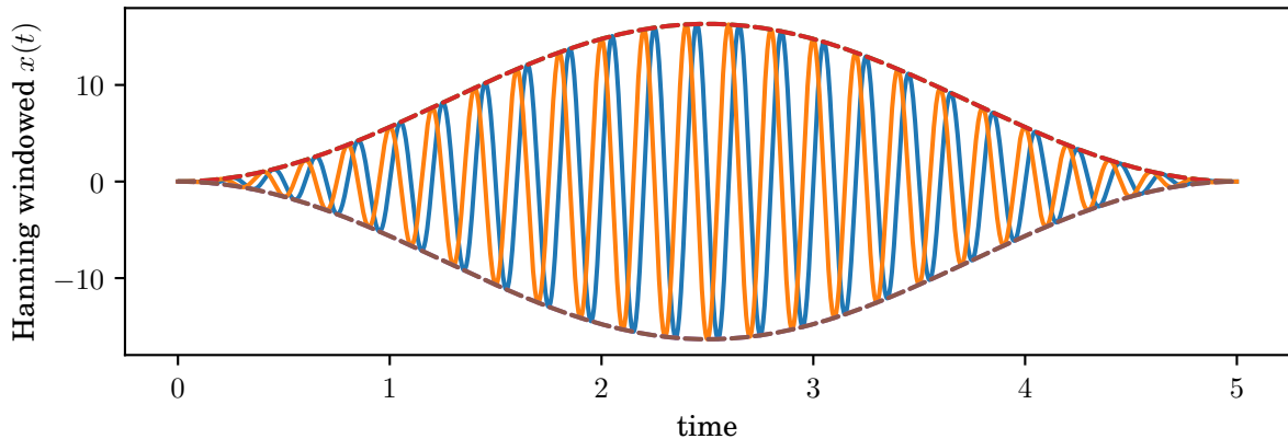
Effect of window. Note the scaling to conserve ASD amplitude
